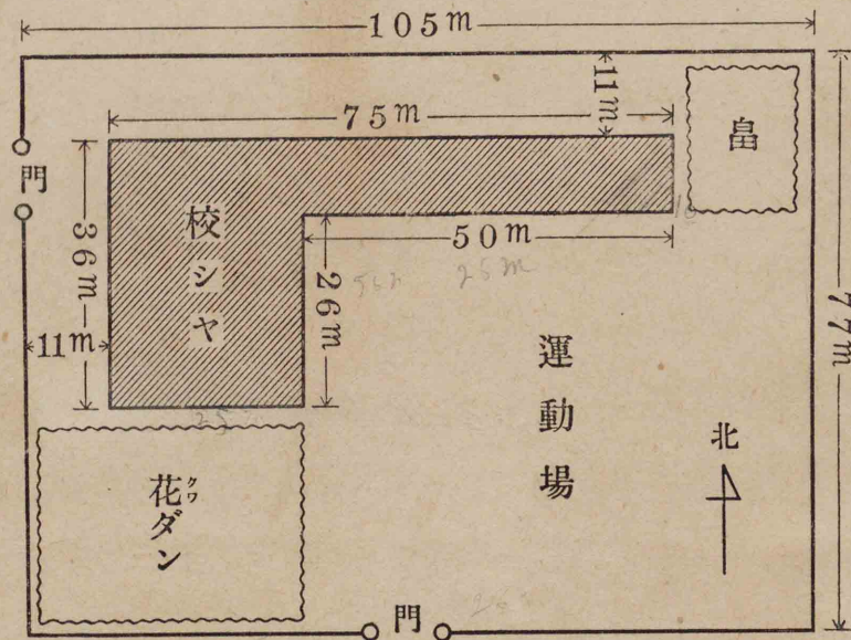
[學校ノ圖面]
